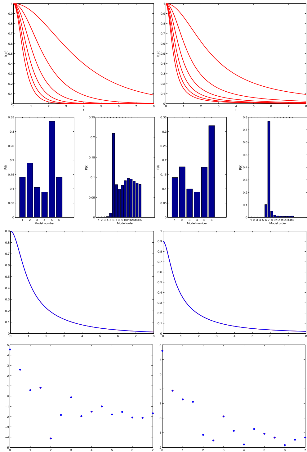
Fig. 5: Left: l = 5 Right: l = 6 a) basis functions b_j(r) , b) p(k|\mathbf{y}) and p(k|\mathbf{y}, \hat{l}) , c) \rho(r) and \hat{\rho}(r) , d) F(q_i) and \hat{F}(q_i) .
